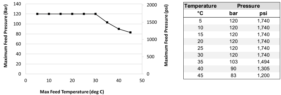
Maximum feed pressure as a function of feed temperature
