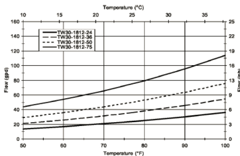
Figure 2: Impact of Temperature on Permeate Flow (constant temperature, recovery)
