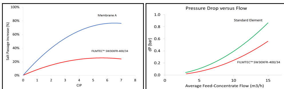
Figure 1: Salt Passage Increase versus number of CIP for SW30XFR-400/34 and Membrane A Figure 2: Element differential pressure versus flowrate for SW30XFR-400/34 and Standard Element
