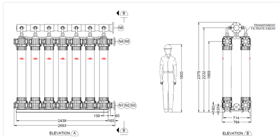
Example: 2x7 - IntegraPac™ IP & IPD-51-14 Arrangement
